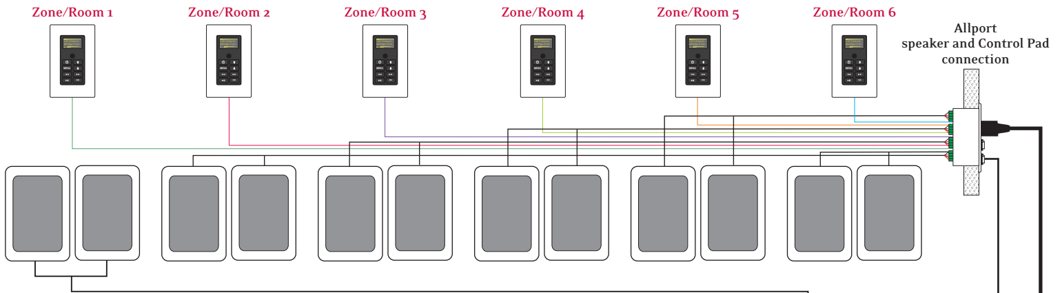
Diagram shown with NuVo NV-P2100 audio amplifiers powering zone 1.
